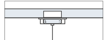
C Powered Canopy Low voltage cable down to fixture from remote driver canopy mounted to junction box
