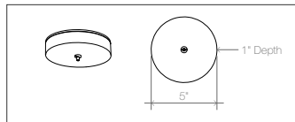
Powered Canopy Driver is in the same room as the fixture
