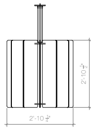
M Linear 2'-10 1/4" Ø x 2'-10 1/2" H
